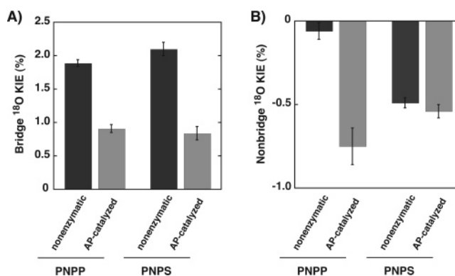
Figure 1. Comparison of KIEs for nonenzymatic and AP-catalyzed reactions of pNPP and pNPS. Values for the 18 O bridge KIEs are plotted in (A), and values for the 18 O nonbridge KIEs are plotted in (B). Isotope effects are expressed as a percentage difference from unity [KIE % = (KIE obs - 1)*100]. Values for nonenzymatic reactions are shown in black, and values for AP-catalyzed reactions are shown in gray.
